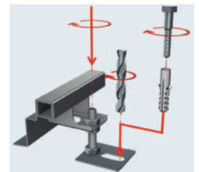
Installation without waterproof membrane
